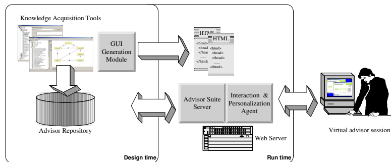
Fig. 1. Architecture of the framework
