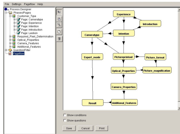
Fig. 2. Modeling the dialogue
